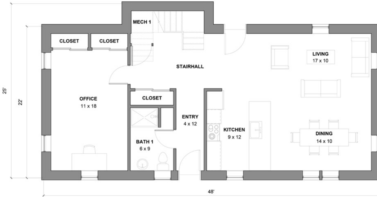
First Floor
